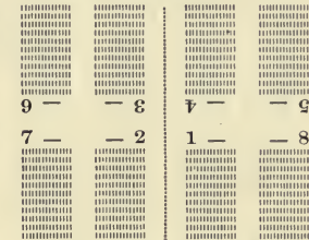
12 Eight pages imposed from the centre.
